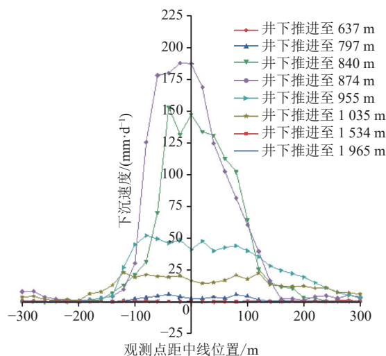
图5 倾向观测线地表下沉速度曲线 Fig.5 Surface subsidence velocity curve of inclined observation line
