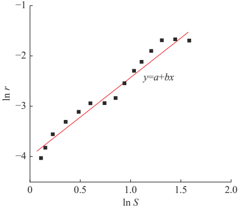
图 11 岩样 5-1-1 \ln S - \ln r 散点图 Fig.11 \ln S - \ln r scatter diagram of 5-1-1 rock sample
