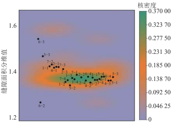
图 10 复合岩层缝隙面积分维值核密度 Fig.10 Fractal dimension value nuclear density of crevice area in composite strata
