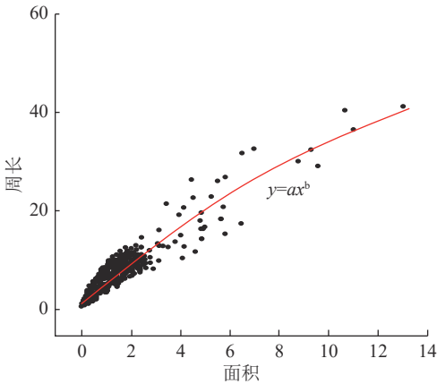
图 9 面积-周长法不同拟合方程及方差 Fig.9 Different fitting equations and variance of area perimeter method
