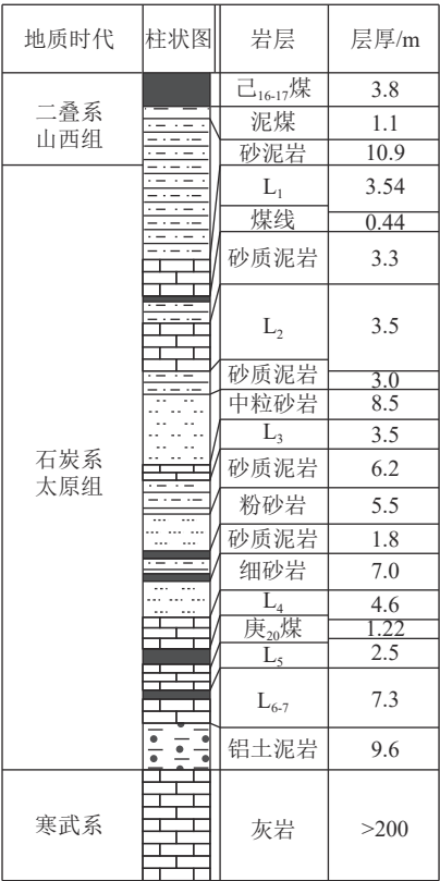
图 1 己 16-17 煤底板复合岩层柱状图 Fig.1 Histogram of 16-17 coal floor composite rock formation
